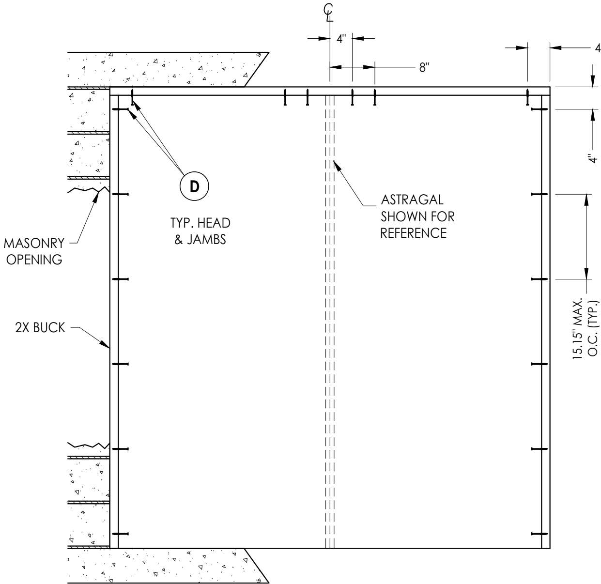
BUCK ANCHORING
