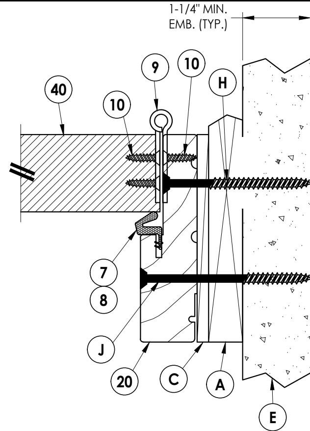
3 HORIZONTAL CROSS SECTION 3 Shown w/1X sub-buck
