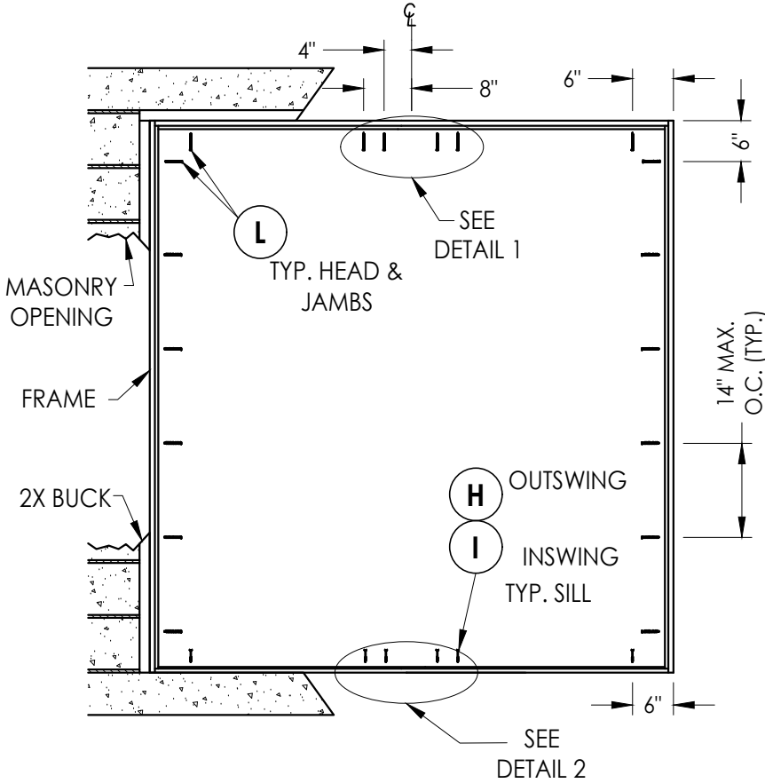
FRAME ANCHORING Masonry 2X buck construction
