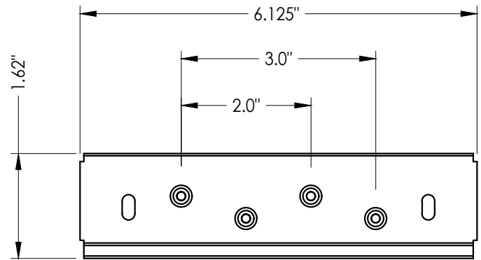
3 HINGE REINFORCEMENT
