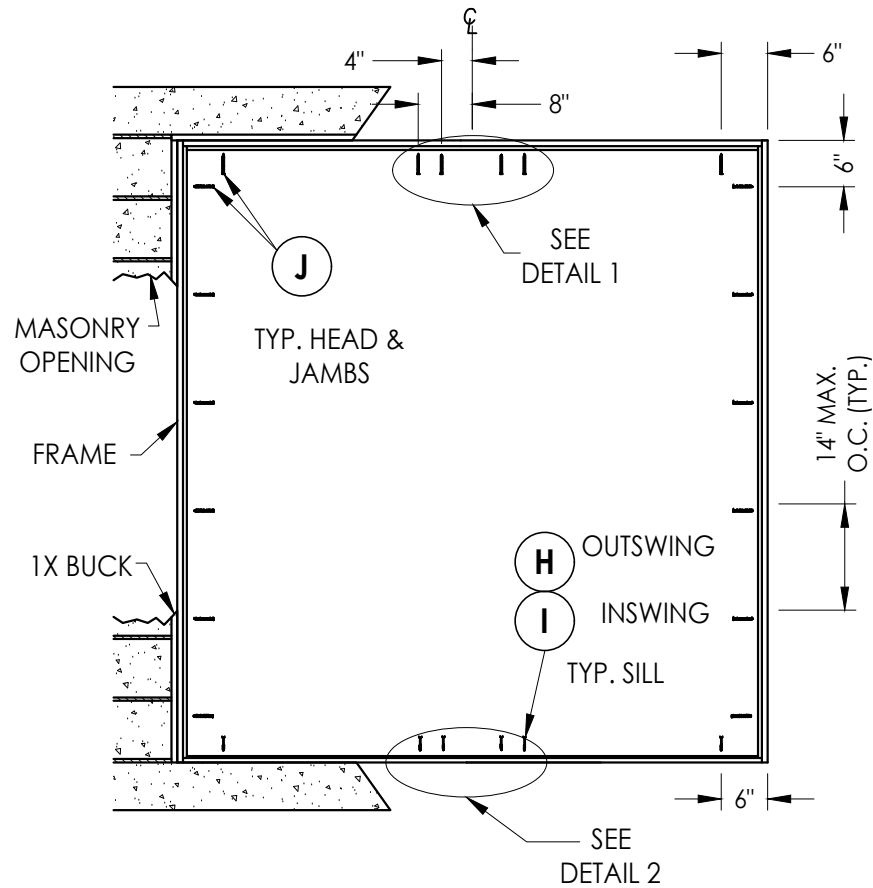
FRAME ANCHORING Masonry 1X buck construction
